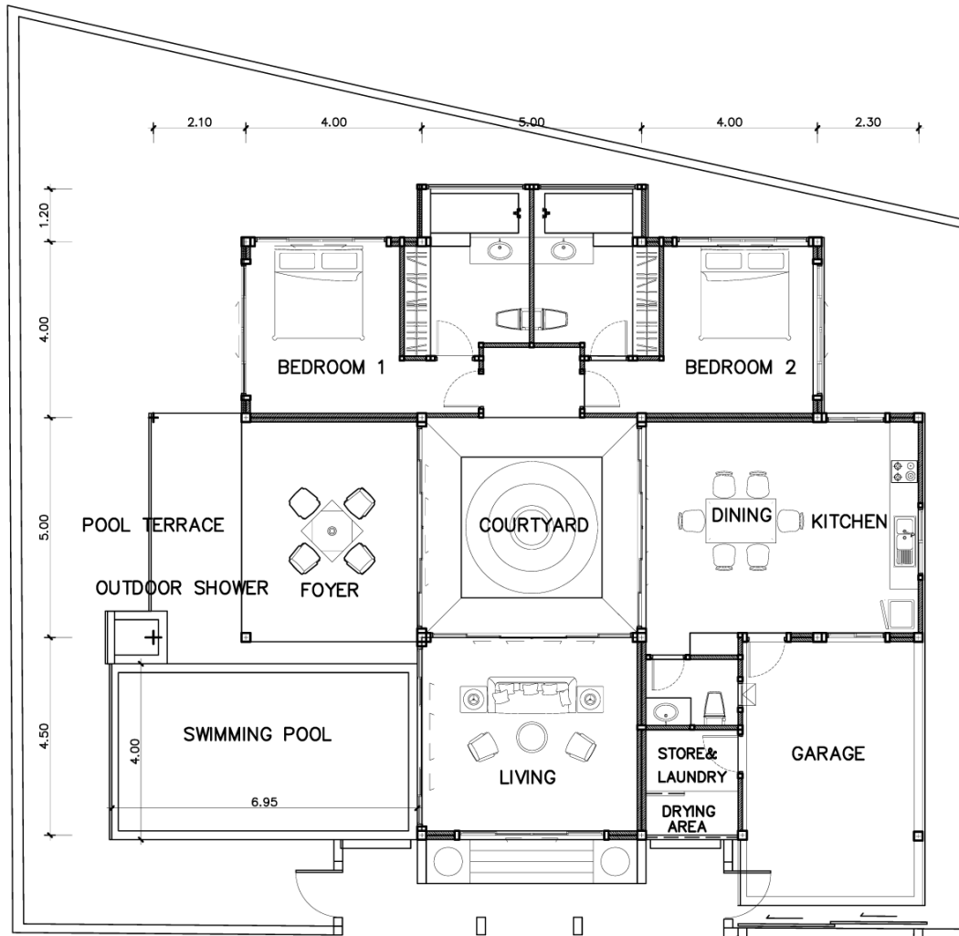
2 BEDROOM TYPE A GROUND FLOOR PLAN
